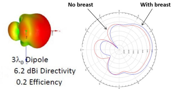
0.44 \lambda_0 Straight & Curved Dipoles in free space
