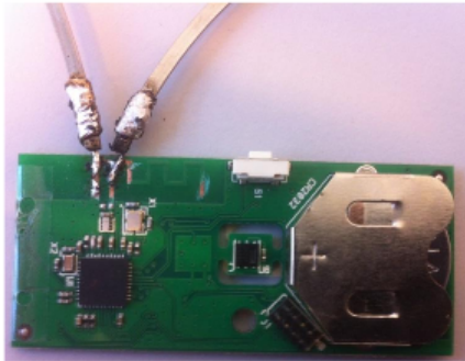
Bra-tenna Integration with TI sensor
