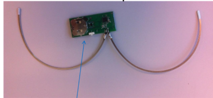
Live test shows 15dB higher RSSI with Bra-tenna versus printed IFA
