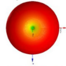
Straight Dipole 2.7 dBi
